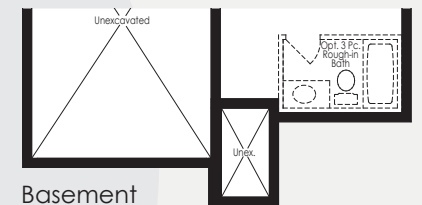
Basement Elevation B
