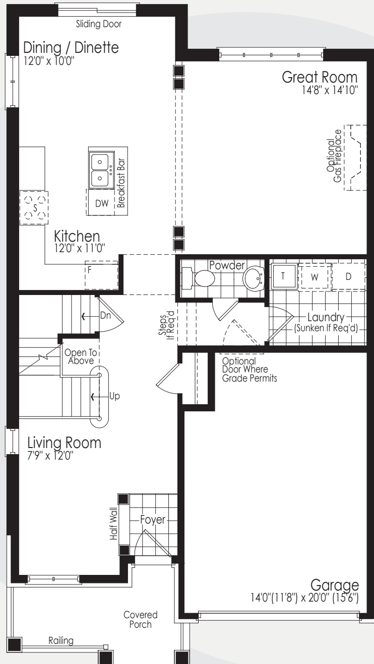
Ground Floor Elevation C & D(Rev)
