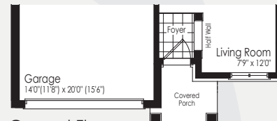
Ground Floor Elevation B
