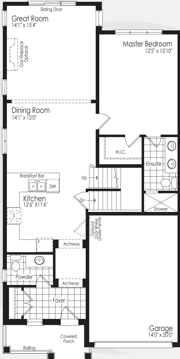
Ground Floor Elevation C
